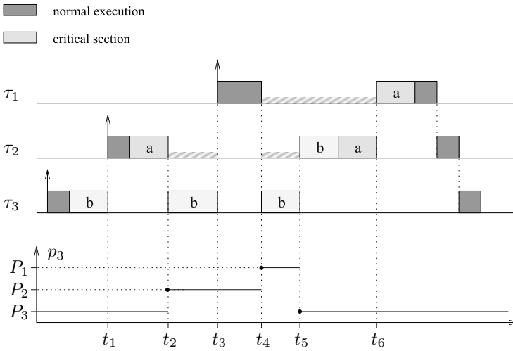
Fig. 7.10 Example of transitive priority inheritance
