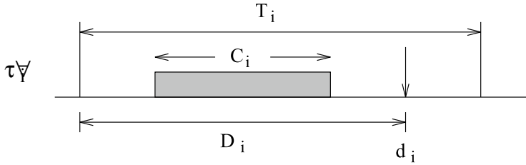
Fig. 4.14 Task parameters in Deadline-Monotonic scheduling
