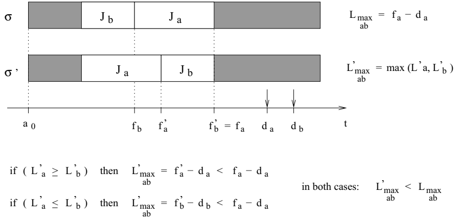
Fig. 3.1 Optimality of Jackson's algorithm
