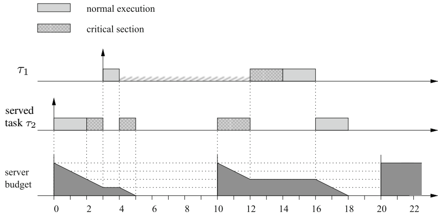
Fig. 9.21 Example of extra blocking introduced when the budget is exhausted inside a critical section
