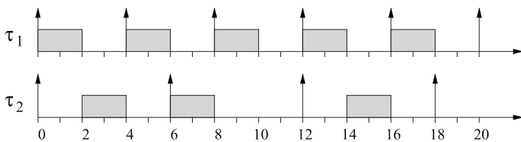
Fig. 4.2 A task set with U_{ub} = 0.9
